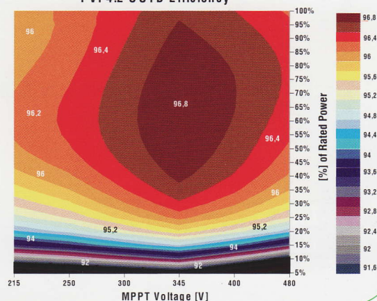
PVI-4.2-OUTD Efficiency
