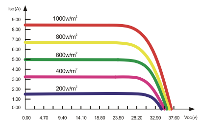
I-V Curves of PV module ZDNY-240C60 at various solar irradiance
