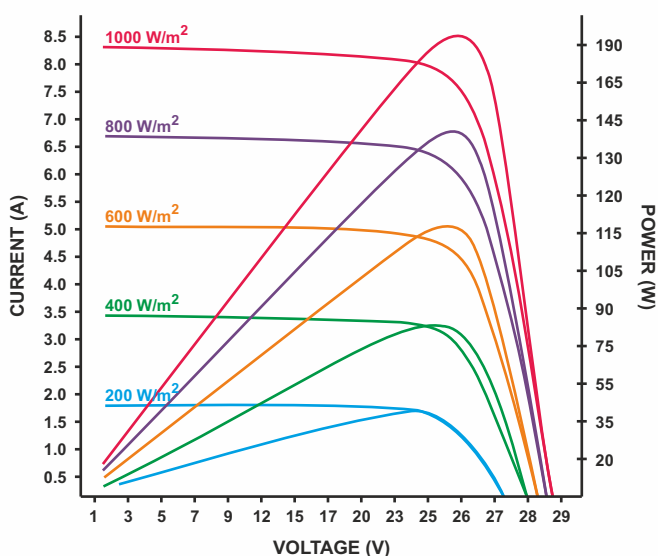
ECO 190 - IV & PMAX GRAPH
