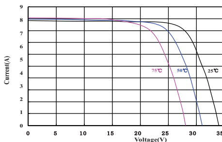
I-V Curves of CNPV-225P-54 at different cell temperature Irradiance: AM.1.5, 1KW/m 2
