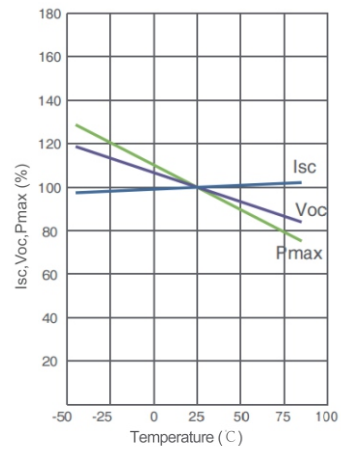
Irradiance:AM1.5,1000W/m²(265W)
