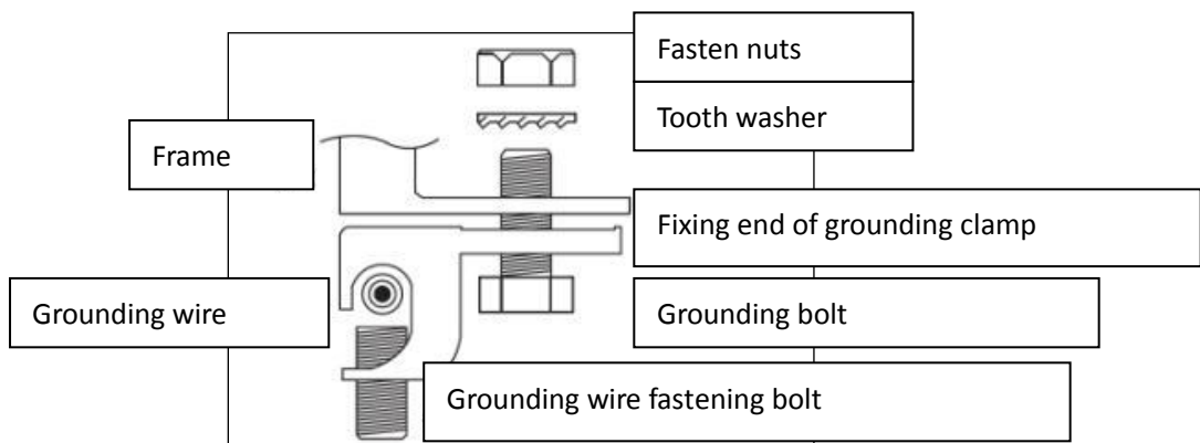
Figure 7 Install Method
